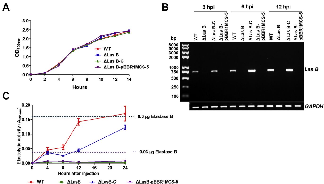
Fig. 4. PAO1 lasB expresses in the hemolymph of silkworm larvae after infection. (A) The growth curves of different PAO1 strains in Luria-Bertani broth. WT, PAO1 wild type; \Delta lasB , lasB deletion mutant; \Delta lasB-C , lasB complemented; lasB -pBBR1MCS-5, \Delta lasB-C control. (B) PAO1 lasB expression after injection into the larval silkworm. The gene expression was analyzed by semi-quantitative PCR with GAPDH acting as an internal control. (C) Elastolytic activity in the hemolymph of PAO1 infected-silkworm larvae. The dash lines represent activity in the hemolymph after injection of purified elastase B.
